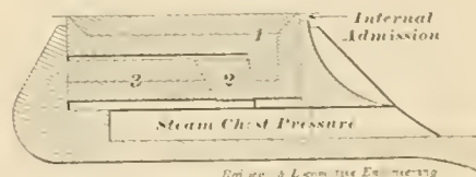
FIG. 17. "AMERICAN" TWO RING—DETAIL.
